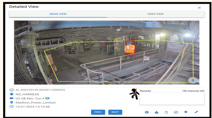
Human Detection
