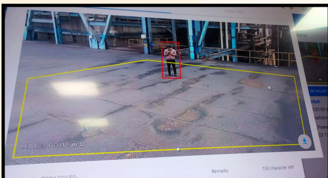
Human Detection
